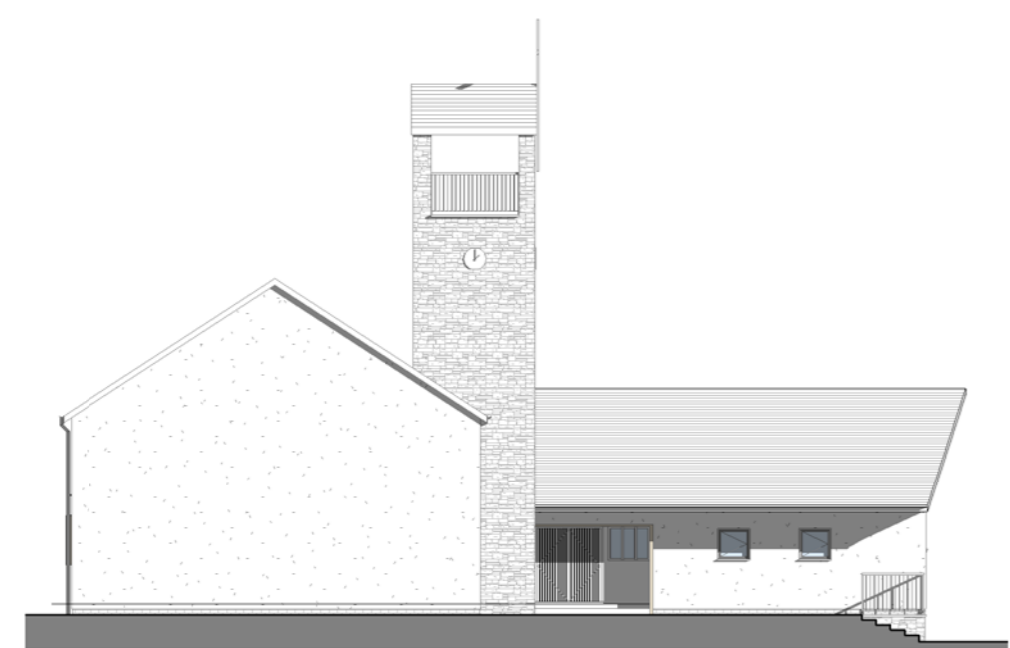
2 Proposed Front Elevation - Church 1:200
