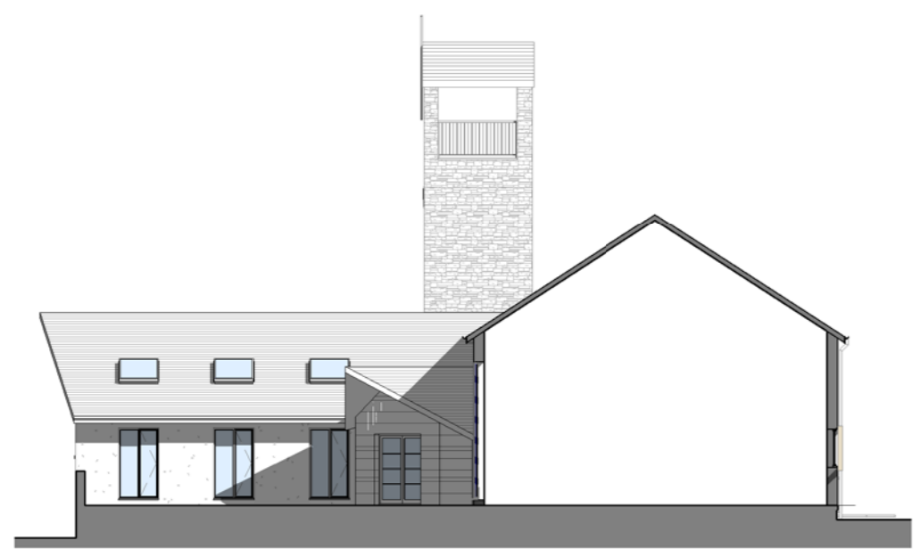
3 Proposed Section Thro Church Hall 1:200
